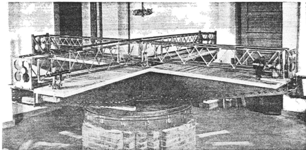
FIG. 10. The Morley-Miller ether-drift interferometer arranged for tests of the Lorentz-FitzGerald hypothesis, 1904.
