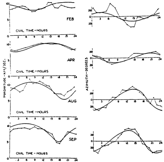
FIG. 27. The observed and calculated velocity and azimuth of ether-drift for the four epochs of observation, plotted with relation to civil time.
