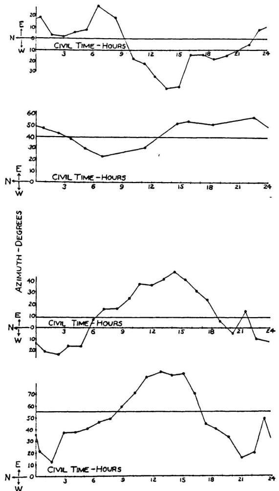
FIG. 25. Chart showing the observed displacement of the axis of azimuth of the ether-drift.
