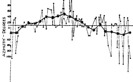
FIG. 22. Single observations and average curves for the ether-drift effect at Mount Wilson in 1925-1926.
