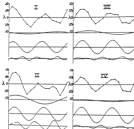
FIG. 21. Harmonic analysis of ether-drift observations.
