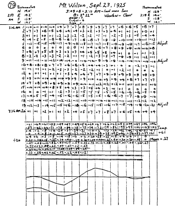
FIG. 8. Form of record of ether-drift observations.
