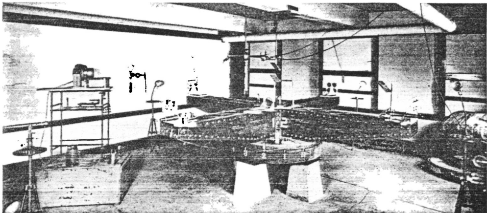
FIG. 14. The interferometer in the laboratory, 1923.
