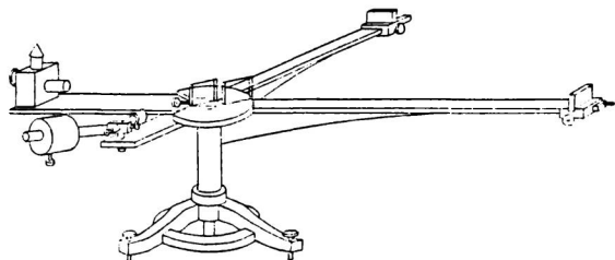
FIG. 1. Michelson's ether-drift interferometer of 1881.
