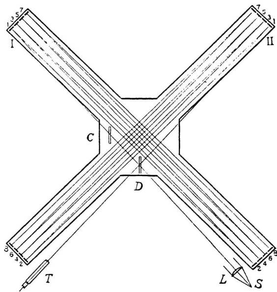
FIG. 6. Plan of the optical paths in the interferometer.
