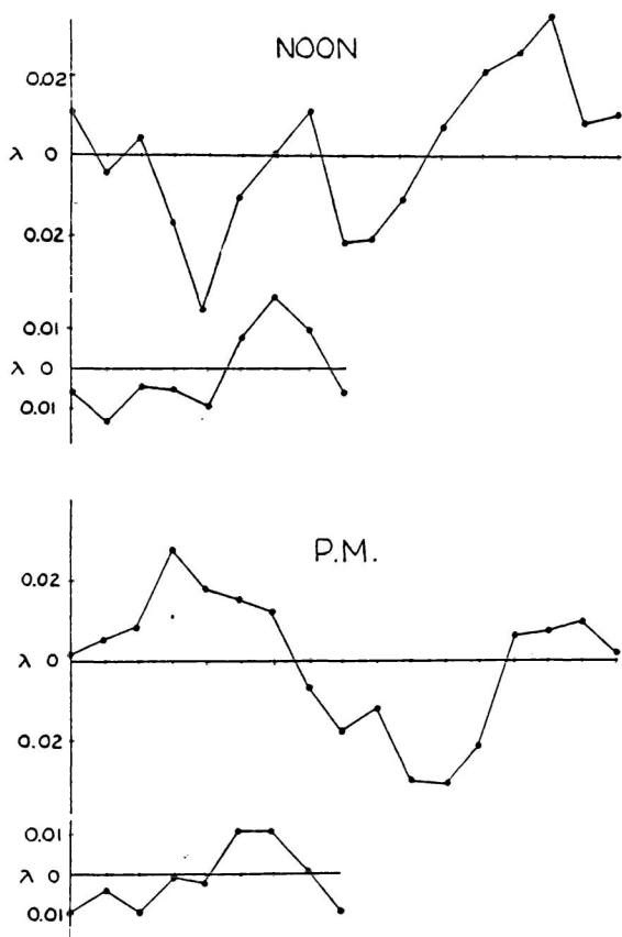
FIG. 3. Fringe displacements of the original Michelson-Morley experiments of 1887.
