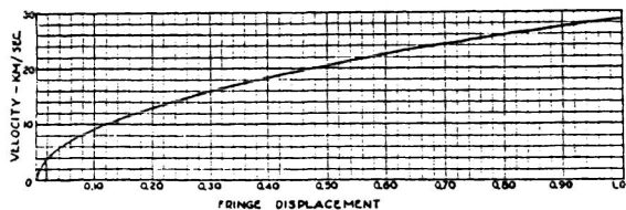
FIG. 20. Relation of fringe displacement to velocity of ether-drift for 2D = 112,000,000\lambda and \lambda = 5700\text{\AA} .
