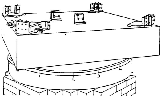
FIG. 2. The Michelson-Morley interferometer of 1887.
