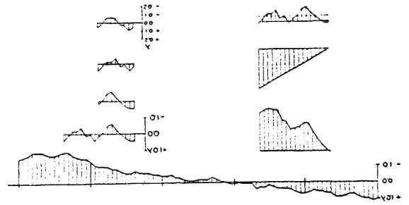
FIG. 9. Interferometer readings and the process of reducing them for the ether-drift effect.
