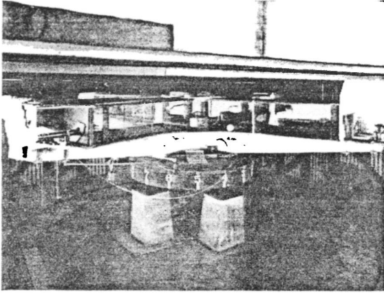
FIG. 13. Interferometer with base of concrete, 1921.
