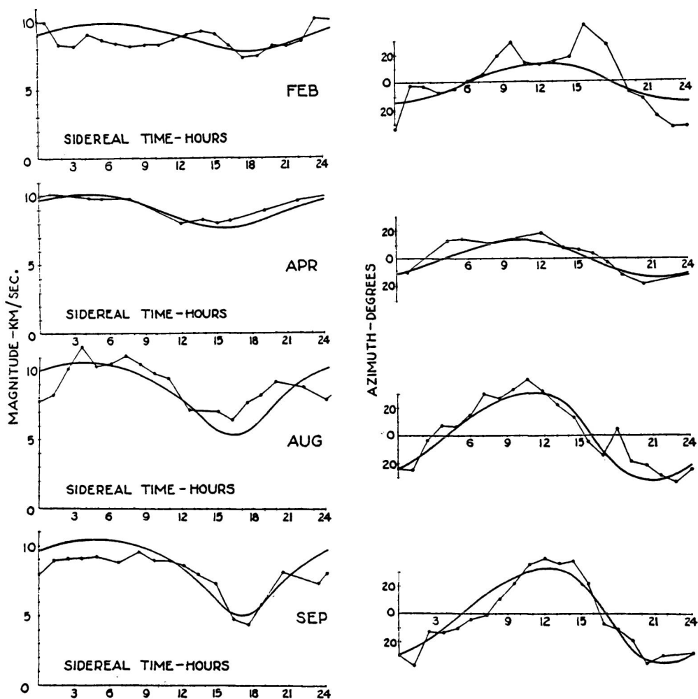
FIG. 26. The observed and calculated velocity and azimuth of ether-drift for the four epochs of observation, plotted with relation to sidereal time.
