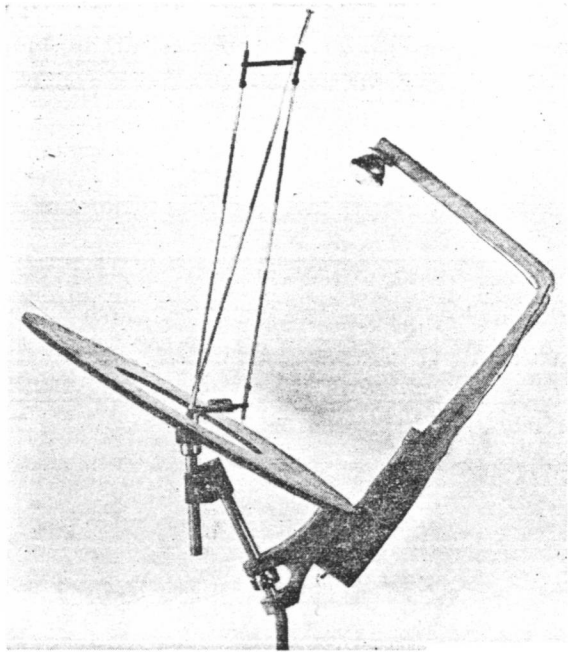
FIG. 18. Model for studying the components of ether-drift.
