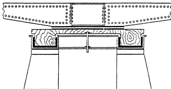
FIG. 5. Cross section of the mercury float for the interferometer.
