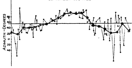
FIG. 22. Single observations and average curves for the ether-drift effect at Mount Wilson in 1925-1926.
